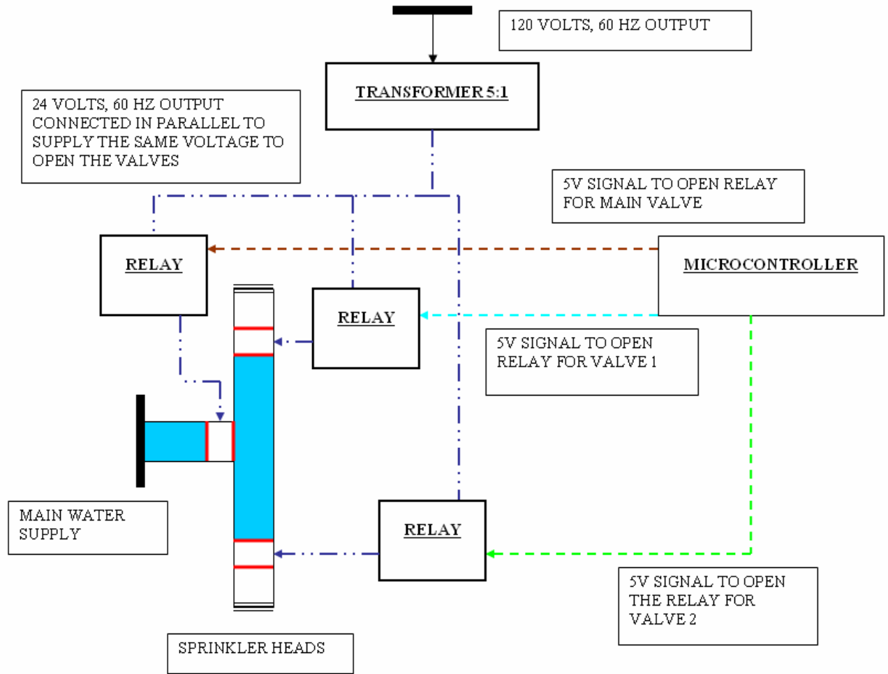
Figure 2: Block diagram of relay circuitry to control valves
