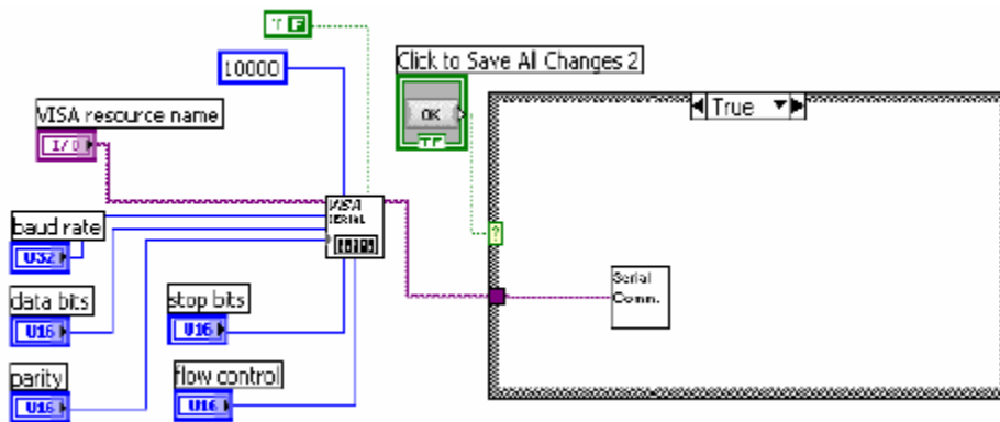
Figure 11 – VI to set up serial communication parameters defined in Figure 10
